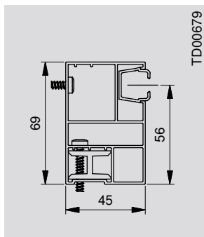
Guida standard 45 x 69 mm
