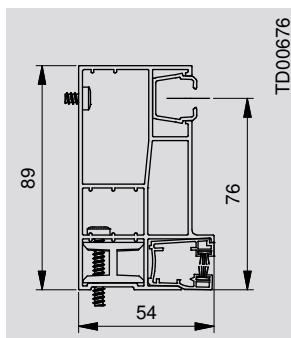
Guida standard 54 x 89 mm
